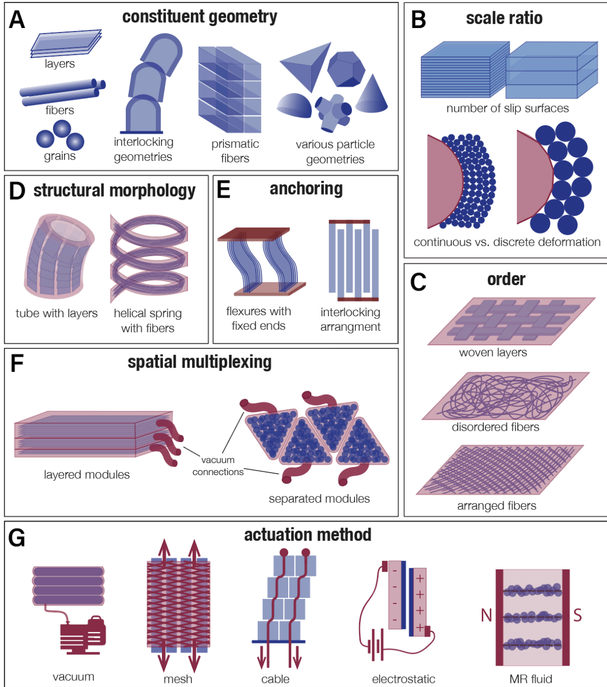
Figure 4. Design parameters of a jamming structure (A) Other than layers, fibers and grains, various constituent geometries can be used to achieve particular mechanical behavior through kinematic constraints. (B) The scale ratio between the constituents and the overall structure impacts both the amount of slip surfaces/lines/points and the way the structure interacts with the scale of application. (C) Constituents can be ordered in varied ways within a structure, to achieve specific anisotropic/isotropic mechanical behavior. (D) The geometry of the overall structure can be used to utilize the high-performing deformation modes of each structure to achieve variable stiffness in the direction of motion. (E) The constituents can be anchored to a system in specific ways, taking advantage of a deformation mode in a particular direction. (F) Multiple airtight envelopes can be brought together to create modules in order to tune the stiffness with higher precision or to separately stiffen and soften different segments of a structure. (G) Other than vacuum, mechanical meshes and cables, electrostatic coupling, and MR fluids can also be used to induce jamming behavior.
