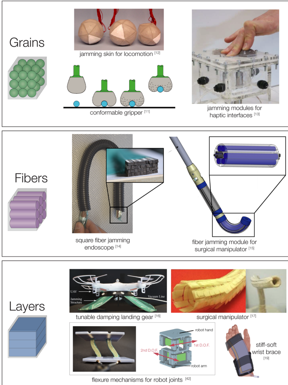
Figure 1. Leading applications of jamming from the literature (A) Granular jamming, with its conformability and isotropic tunable stiffness, has been used for locomotion, grasping and haptic interactions. (Image copyright information, from left to right: Reprinted with permission from [11] , © 2010 IEEE. Reprinted, with permission, from [12] , © 2013 IEEE. Reprinted, with permission, from [13] ) (B) Fiber jamming, with its ability to provide multi-directional variable bending stiffness in long and slender elements, has been used for medical applications, such as endoscopes and surgical manipulators. (Image copyrights, from left to right: © 2020 IEEE. Adapted with permission from [14] , © 2019 Brancadoro, Manti, Grani, Tognarelli, Menciassi and Cianchetti. Adapted from [15] ) (C) Layer jamming, with its unidirectional variable bending stiffness, has been used for a variety of applications such as landing gear, surgical manipulators, joints for rigid robots and wearables: (Image copyright information, from left to right. Upper row: © 2017 IEEE. Reprinted, with permission, from [16] , © 2013 IEEE. Reprinted, with permission, from [17] , Lower row: : © 2019 IEEE. Reprinted, with permission, from [42] , © 2020 IEEE. Reprinted, with permission, from [19] )
