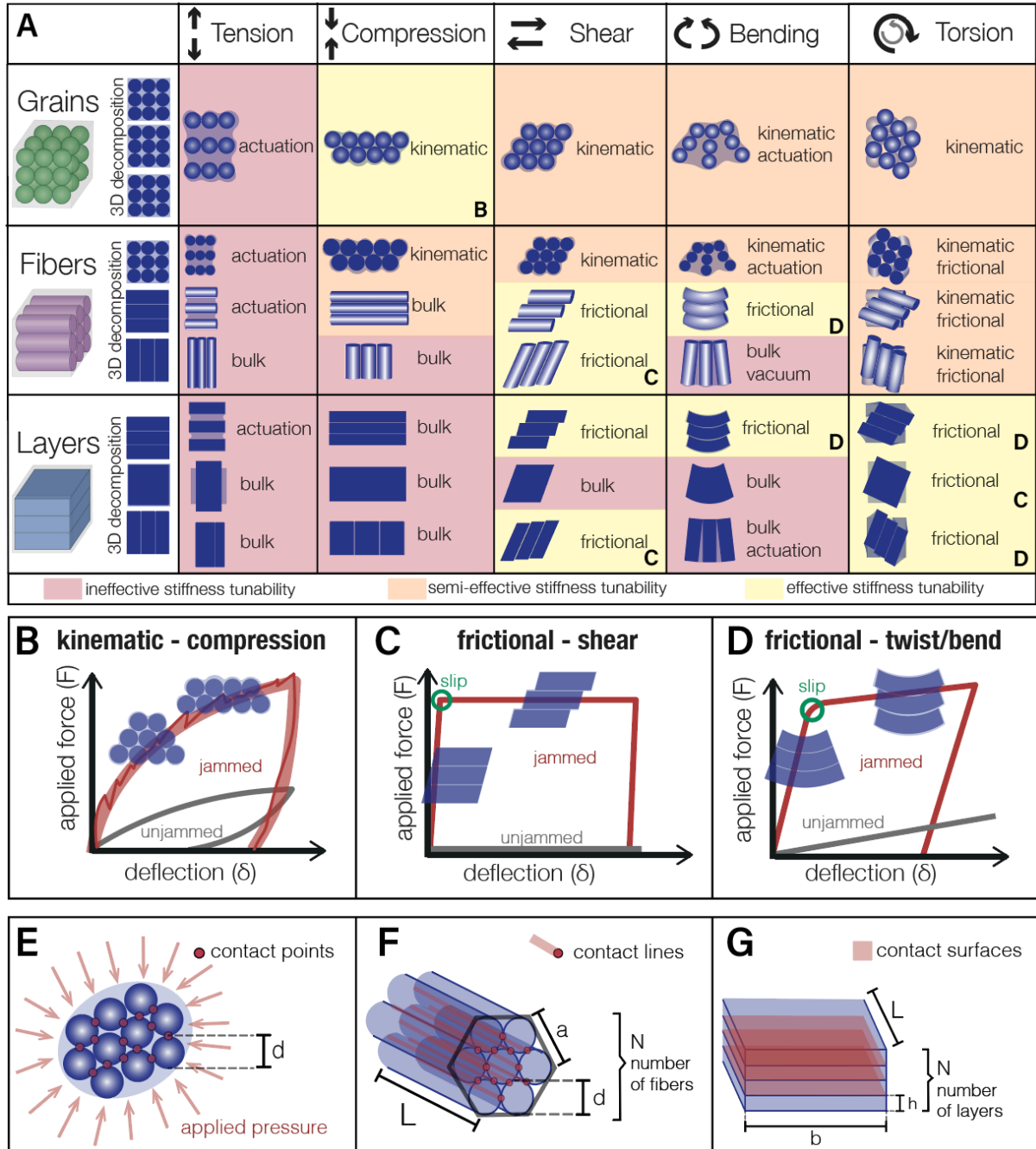
Figure 3. Deformation modes of elementary jamming structures (A) The deformation mode governing the jamming structure for each type of media (grain, layer, fiber) under each fundamental loading condition is shown. (See Supplementary Video SV1.) (B) Representative force-deflection curve for the kinematic deformation mode. [11,40] Note that there is typically non-monotonic behavior (shown with the thin dark red line) due to localized geometric rearrangements. (C) Representative force-deflection curve for the frictional mode in which the applied force only causes sliding between the constituents. [20,34] (D) Representative force-deflection curve for the frictional deformation mode in which there is not only sliding, but also bending and/or twisting. [9,10,14,19] (E-G) Contact geometries for jamming structures with grains, fibers, and layers are respectively points, lines and surfaces.
