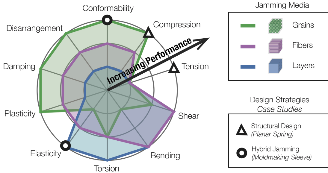
Figure 7. Design space of jamming structures based on performance metrics. The spider plot shows how the design space is spanned by the three different jamming media, giving designers and engineers the opportunity to choose the right jamming media for a particular application. The case studies presented in the previous section are presented as data points to show how the proposed design strategies expand the design space: combining grains and layers to achieve both conformability and elasticity, and designing a planar spring to achieve variable stiffness under tension and compression.
