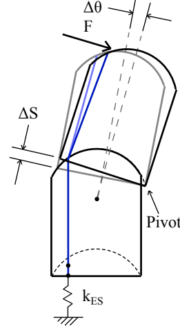
Fig. 6. Elastic structural deformation kinematics.
