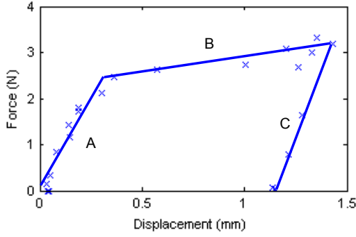
Fig. 5. Typical force vs. displacement during catheter tip contact. Schematic line A results from elastic structural deformation. Schematic line B results from sliding friction. Schematic line C results from relaxation of elastic deformation.
