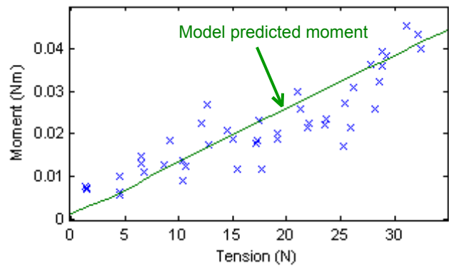
Fig. 10. Moment applied to catheter tip creates sliding displacement as a function of the total pull wire tension. Line represents the model estimated moment to cause sliding.
