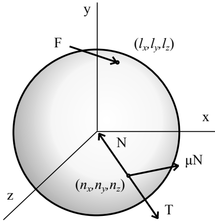
Fig. 7. Diagram of forces acting during sliding displacement.
