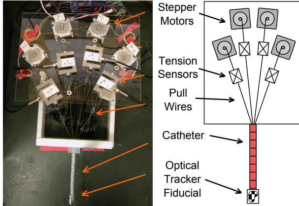
Fig. 8. (left) Photo and (right) diagram of catheter stiffening robot system (view from top).
