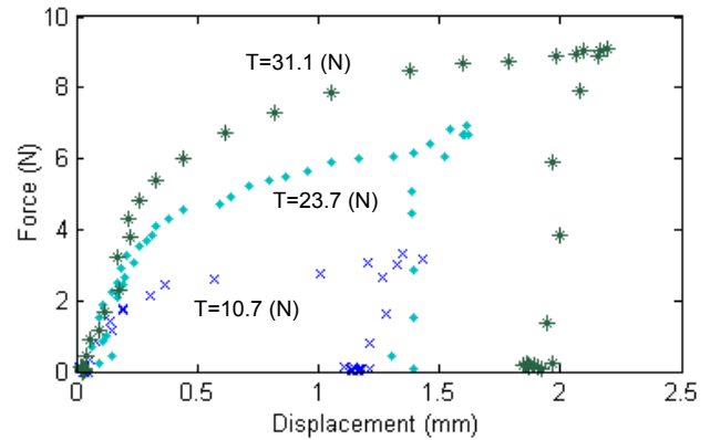
Fig. 9. Moment applied to catheter tip creates sliding displacement for three different pull wire tensions.
