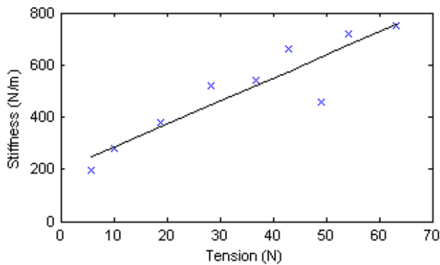
Fig. 11. Overall catheter stiffness before sliding as a function of the total pull wire tension (10 vertebrae). Black line represents linear fit.
