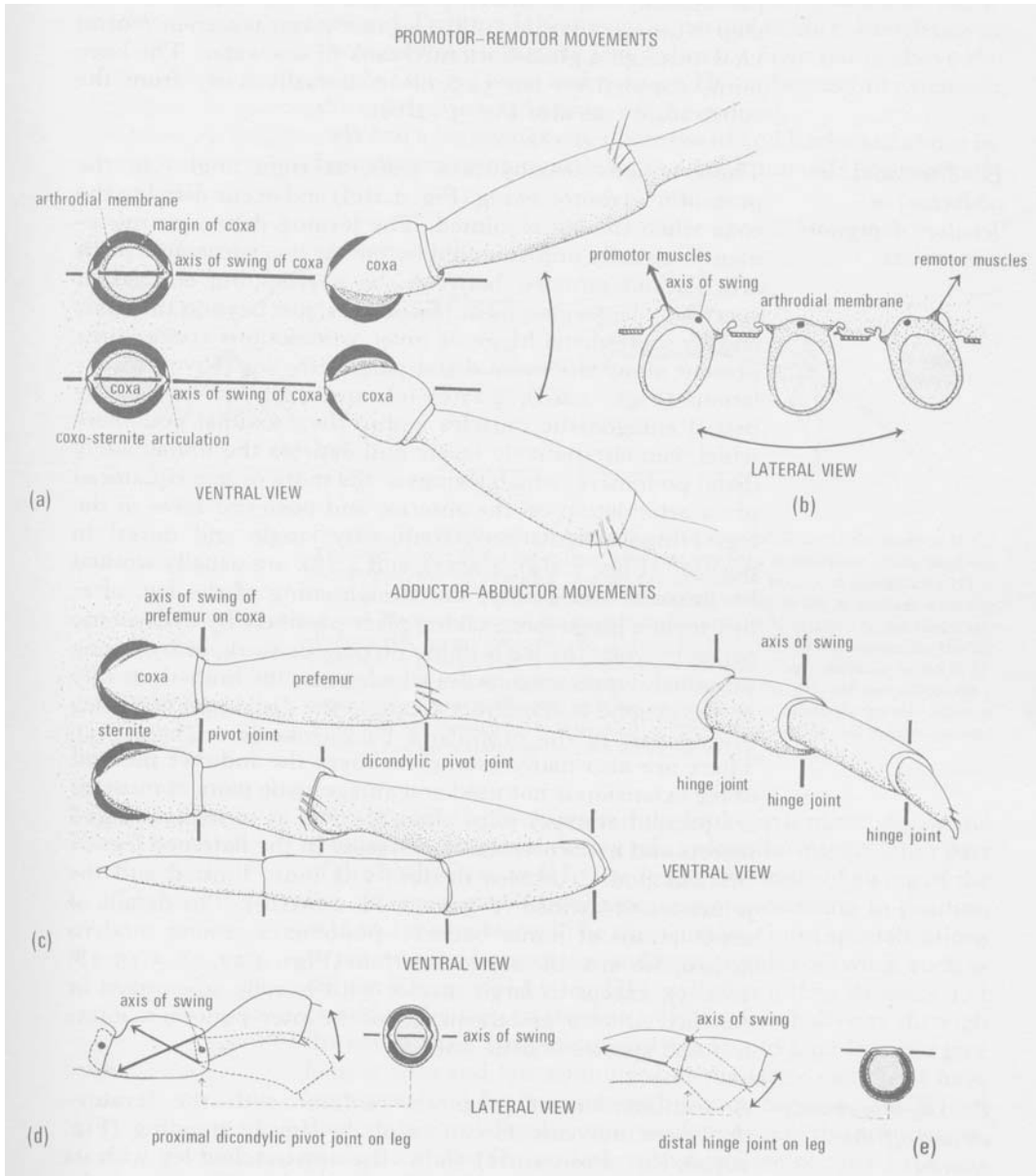
Figure 2: Joint analysis of a typical arthropod leg [Manton, 1977, p. 41]
