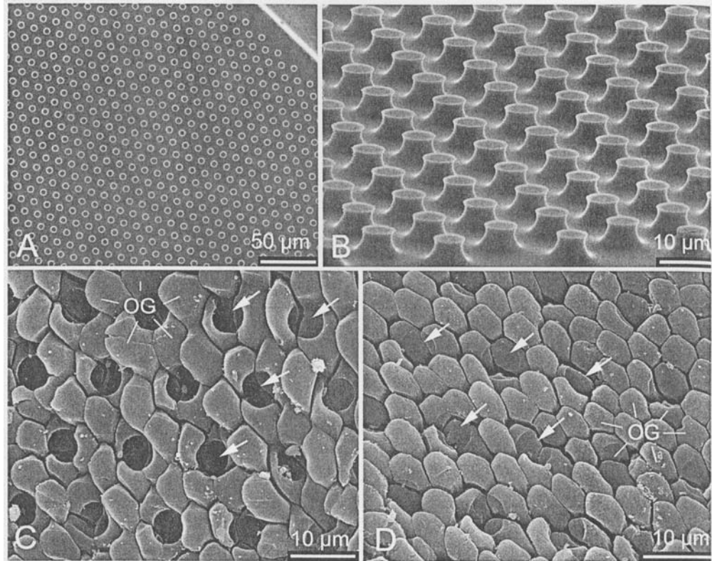
Figure 24: SEM views of Silicon substrate (A and B) and the attachment pads of the great green bush cricket when standing on the substrate (under strong load (C) and light load (D)) [Gorb et al., 2000, p. 826]
